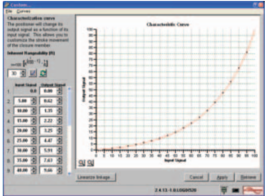
Figure 8: Manual Tuning with User Interface
