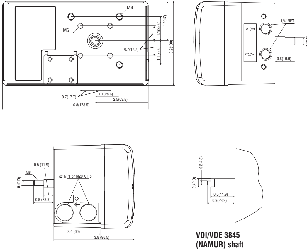
Figure 18: Logix 500si Digital Positioner Dimensional Drawings
