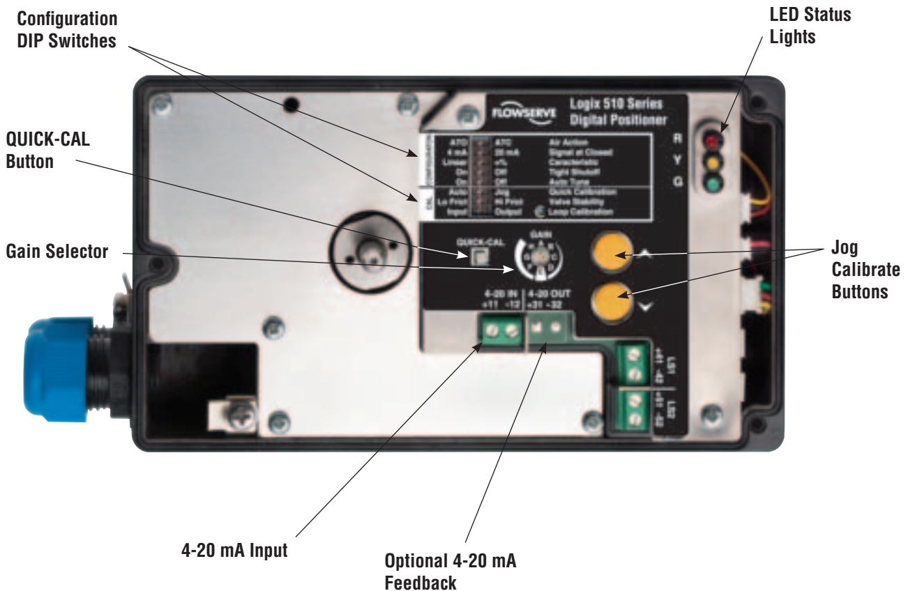
Figure 2: Logix 510si Digital Positioner
