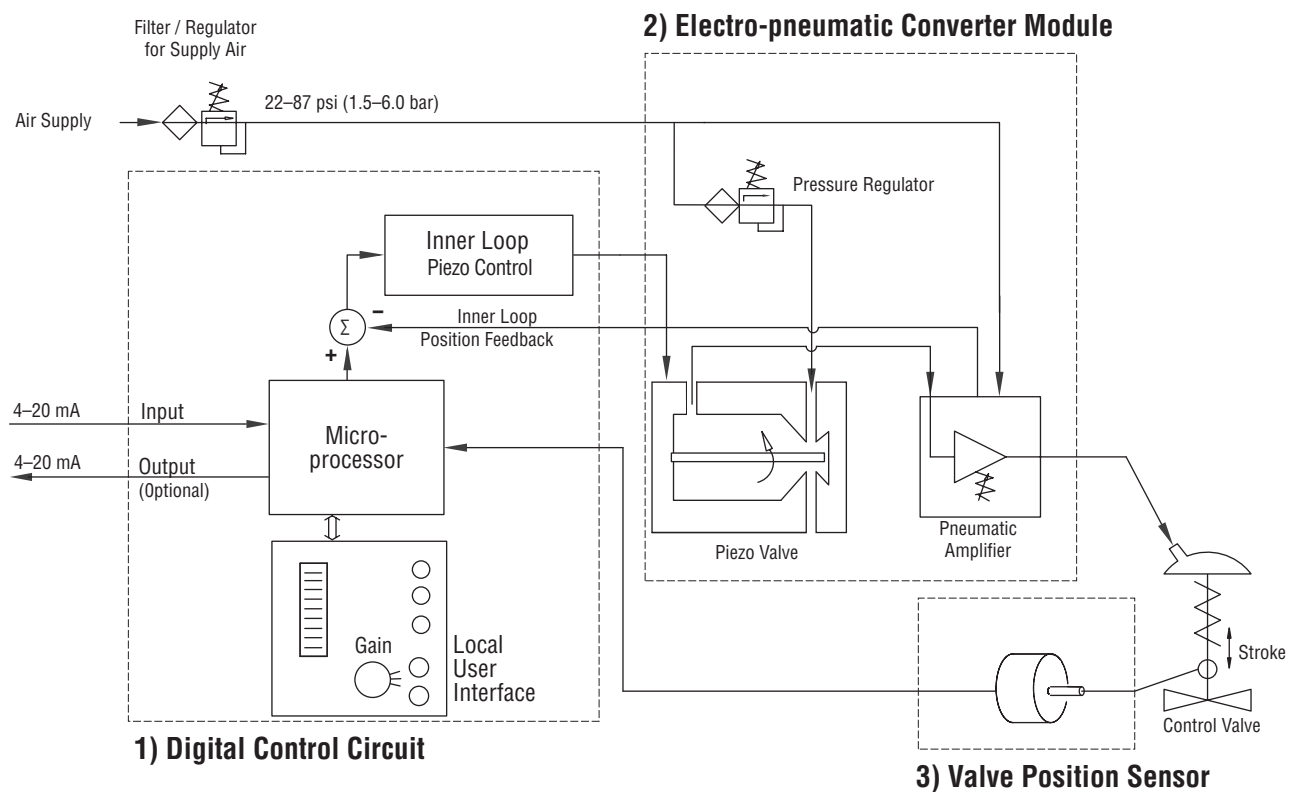
Figure 3: Logix 510si Digital Positioner Schematic
