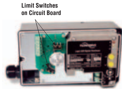
Figure 12: Optional Internal Limit Switches
