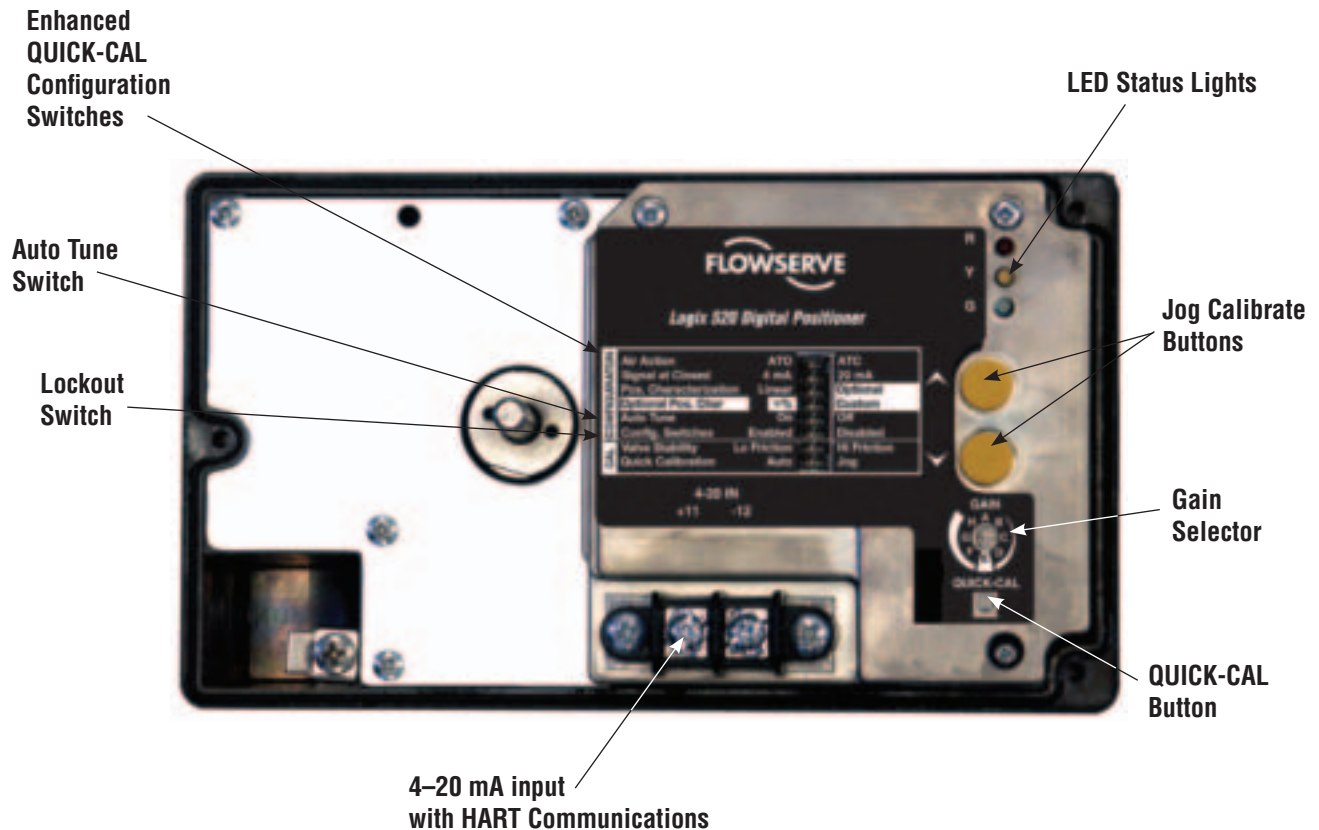
Figure 4: Logix 520si Digital Positioner
